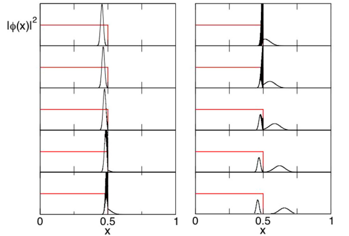
Fig. 3. Numerical simulation of the time-dependent Schrödinger equation for the hard step potential of Eq. (1). The picture shows ten snapshots of |\psi|^2 (black lines) at different times before, during, and after passing the potential step (order: left column top to bottom, then right column top to bottom). The straight lines in the figures depict the potential in arbitrary units. It can be seen that there is a transmitted wave packet and a reflected wave packet. The initial wave function is a Gaussian wave packet centered at x=0.4 with \sigma=0.01 and k_0=500\pi . The simulation assumes infinite potential walls at x=0 and x=1 . The step height is \Delta=15E , and the x -interval is resolved with a linear mesh of N=10^4 points. The snapshots are taken at times 6, 7, 8, ..., 15 in appropriate time units.
